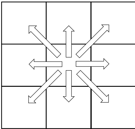
Figure 8. Queen's contiguity.
